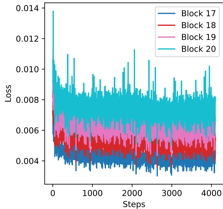
Loss for Blocks 17 to 20
