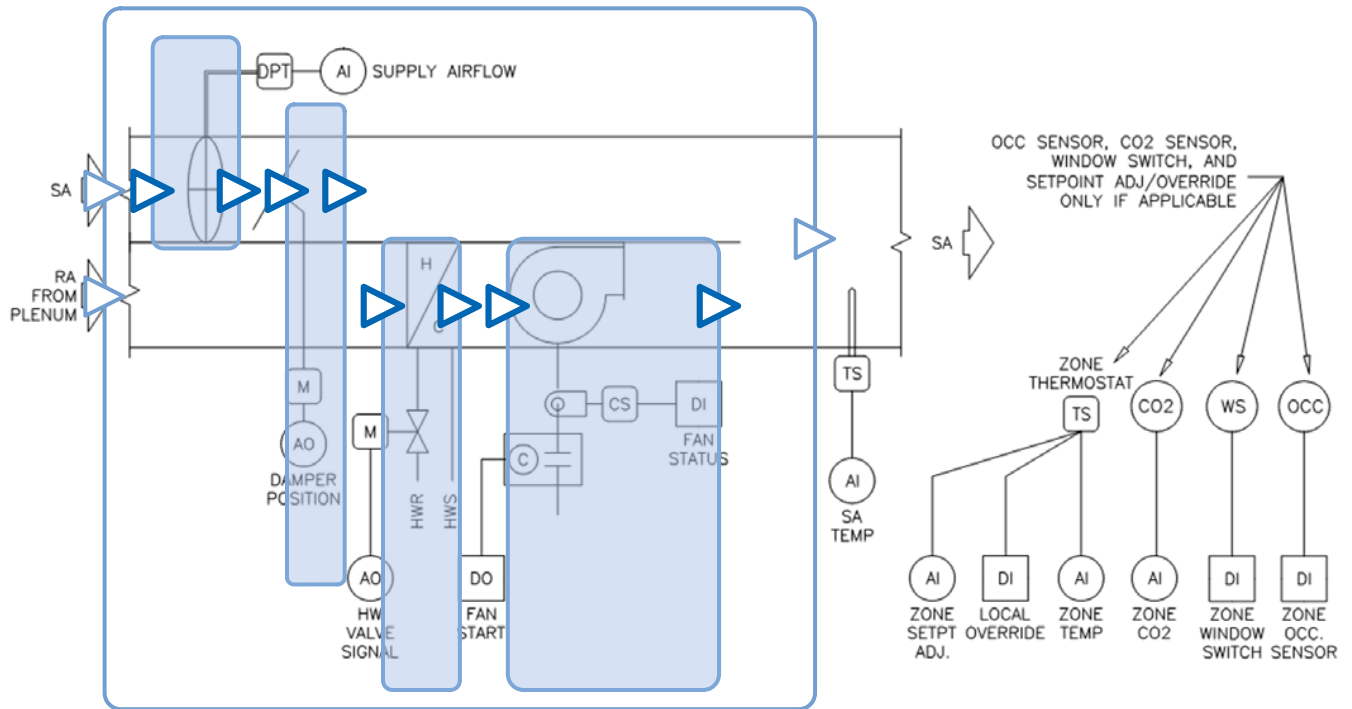
Connection points for devices
