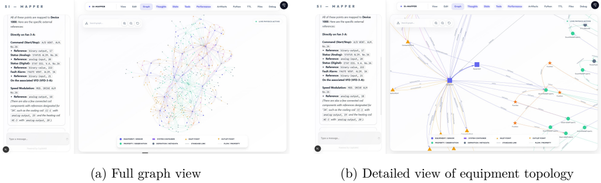
Figure 7: System 3 — generated ASHRAE 223P semantic graph in the SI-Mapper Neo4j visualization. The detailed view shows equipment nodes with connection points, medium types, and BACnet external references.
