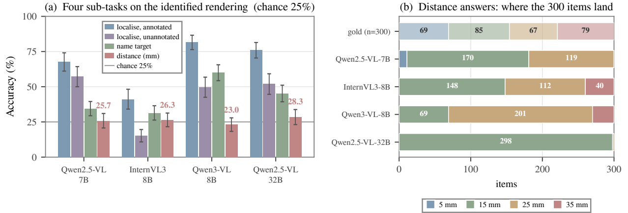
Fig. 7. Perception works, naming partly works, metric estimation is absent. (a) Sub-task accuracy on the identified rendering with volume-clustered 95% intervals: which organ holds the red-outlined lesion, the same with outlines and legend removed, which structure is outlined in cyan, and how many millimetres separate them. (b) Where the 300 distance answers land against the near-uniform gold: every model collapses onto one or two buckets, Qwen2.5-VL-32B onto “15” for 298 items.
