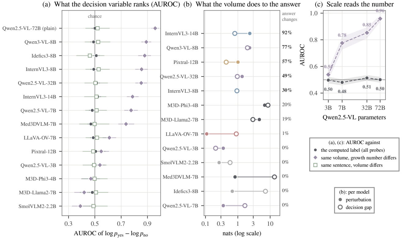
Fig. 7. The decision variable reads the question, not the volume. (a) AUROC of \log p_{\text{yes}} - \log p_{\text{no}} on the growth-matched subset with volume-clustered 95% intervals: against the computed label over all 1,368 probes; within the 363 complete matched pairs, where volume and rendering are identical and only the growth number in the question differs; and across the 182 probes whose question sentence is identical and only the volume differs. (b) Mean log-probability perturbation between sighted and blind arms (filled) against the sighted-arm decision gap (open), sorted by the share of probes whose answer changes. (c) The label and within-pair AUROCs across Qwen2.5-VL 3B–72B on the published rendering.
