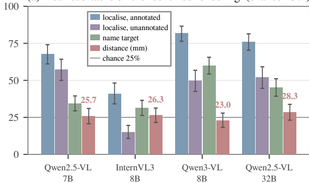
(a) Four sub-tasks on the identified rendering (chance 25%)
