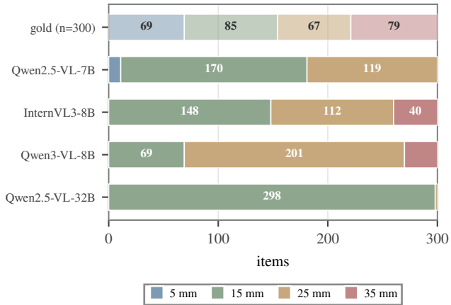
(b) Distance answers: where the 300 items land
