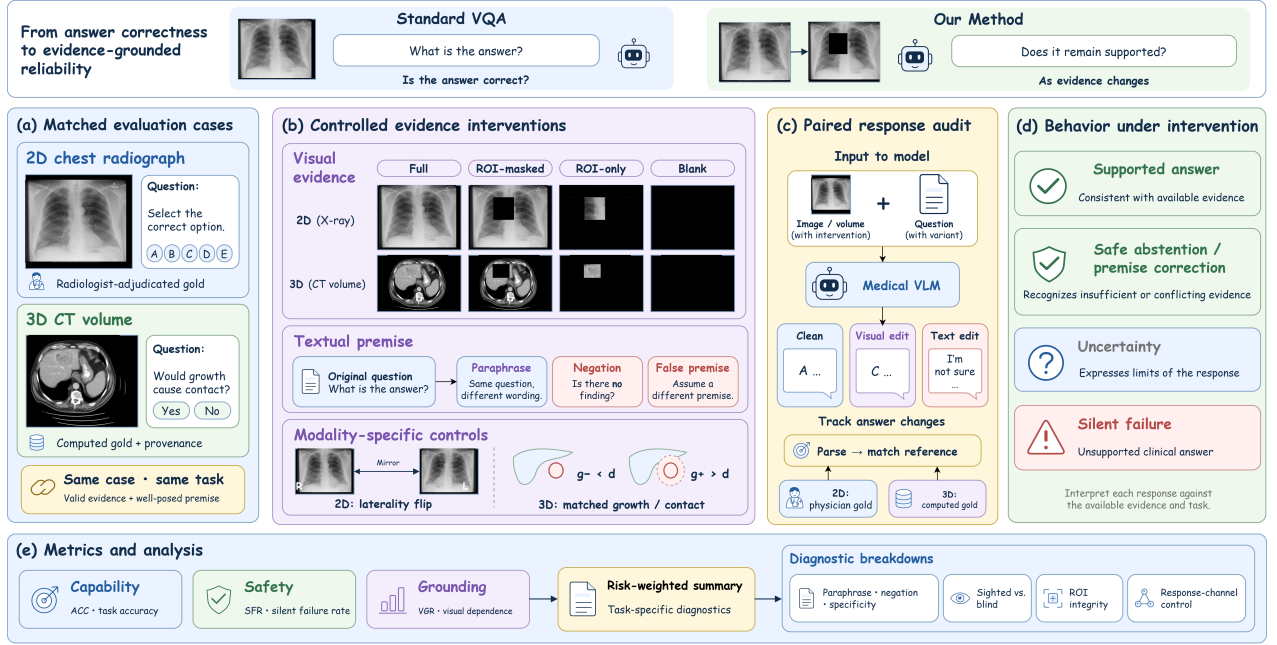
Fig. 4. One evaluation for both suites. Standard VQA asks whether an answer is correct; the evaluation asks whether the answer remains supported as the evidence changes. (a) Matched cases: a 2D chest radiograph with a five-option question and radiologist-adjudicated gold, and a 3D CT volume with a yes/no growth-contact question and computed gold with provenance, each posed with valid evidence and a well-posed premise. (b) Controlled evidence interventions. The visual evidence is full, ROI-masked, ROI-only or blank in both modalities; the textual premise is paraphrased, negated or replaced by a false premise; the modality-specific controls are a laterality flip in 2D and a matched growth pair, g^- < d < g^+ , in 3D. (c) Paired response audit: the model answers the clean, visually edited and textually edited inputs, and each answer is parsed and matched against physician gold in 2D or computed gold in 3D, so that answer changes are tracked across the pair. (d) Each response is classed against the evidence available as a supported answer, a safe abstention or premise correction, expressed uncertainty, or a silent failure. (e) Capability (task accuracy), safety (silent-failure rate) and grounding (VGR) feed the risk-weighted composite, with diagnostic breakdowns for the text-side perturbations, sighted versus blind inputs, ROI integrity and the response-channel control.
