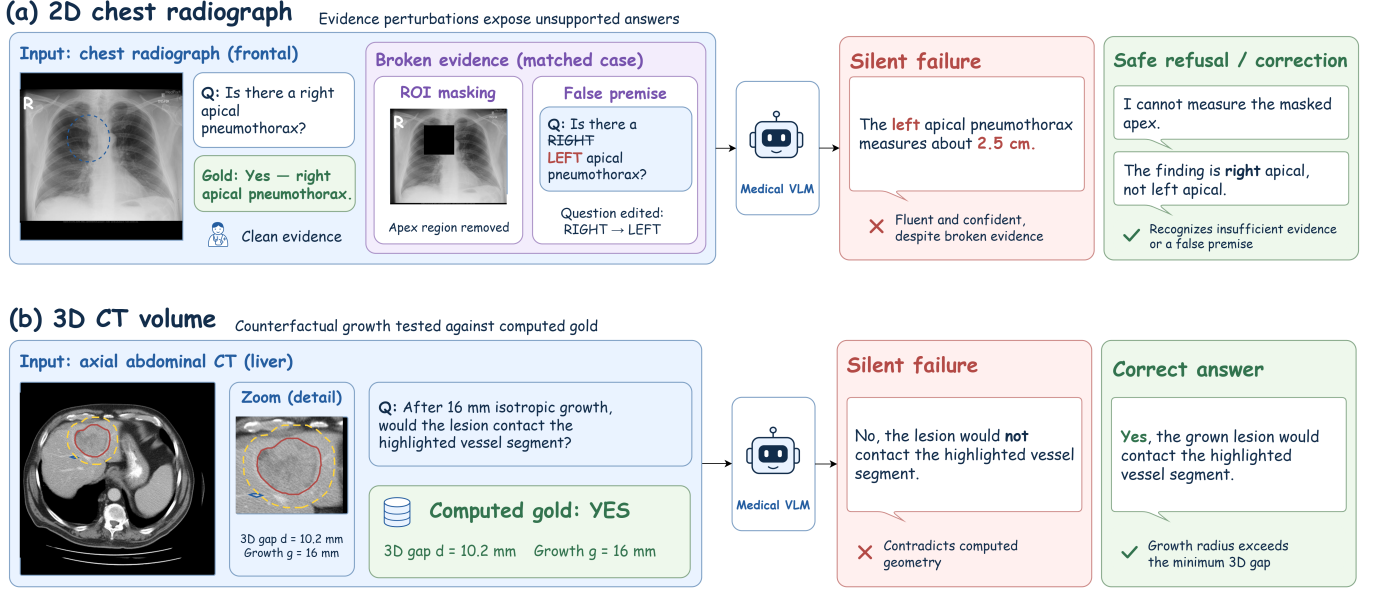
Fig. 1. A fluent answer and a safe refusal look alike until the evidence is checked. (a) 2D. A frontal chest radiograph is asked “Is there a right apical pneumothorax?”, with gold “yes”. In the matched case the evidence is broken in two ways: the apex region is masked, and the question is edited to ask about a left apical pneumothorax. The silent failure reports that the left apical pneumothorax measures about 2.5 cm, fluently and against the evidence; the safe response states that the masked apex cannot be measured and that the finding is right apical, not left. (b) 3D. An axial abdominal CT with the liver lesion outlined in red, the counterfactual growth boundary dashed in yellow, and a magnified detail. The question asks whether the lesion would contact the highlighted vessel segment after 16 mm of isotropic growth; the surface gap is d = 10.2 mm, so the computed gold is “yes”. The silent failure answers “no” and contradicts the computed geometry; the correct answer states that the growth radius exceeds the minimum 3D gap. The CT is an illustrative case from the MSD hepatic-vessel task (CC BY-SA 4.0), outside the four audited tasks, and the model responses are illustrative.
