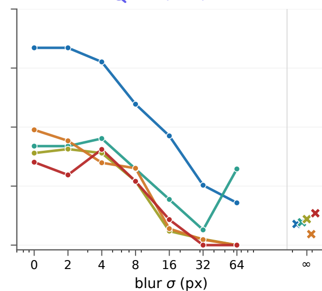
Qwen3.5-397B
