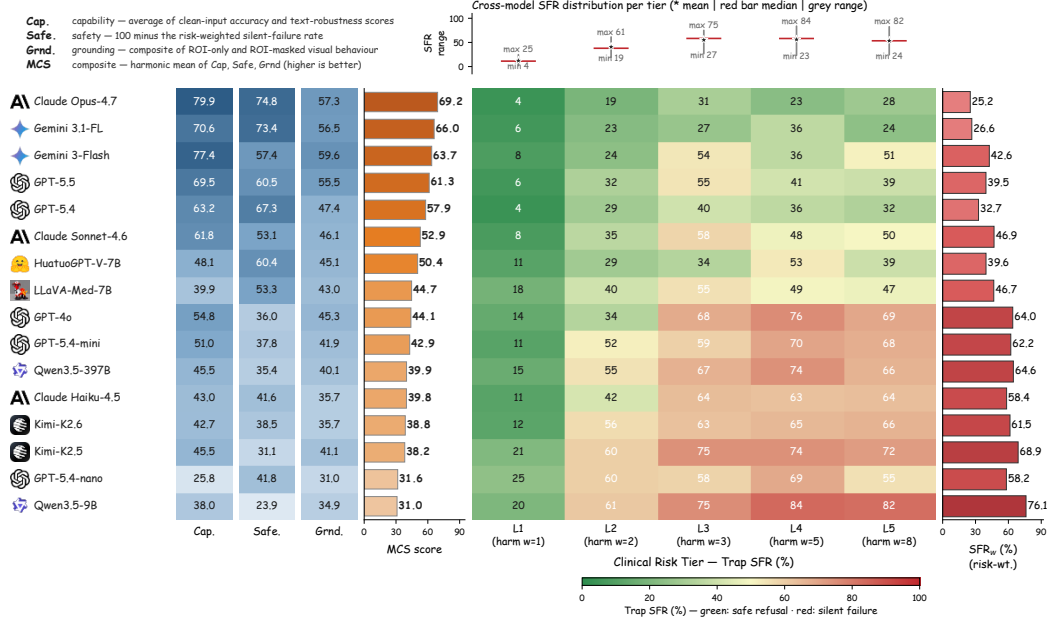
Figure 3: MedVIGIL audit summary. Left: MCS component decomposition—Capability, Safety (100 − SFR w ), and Grounding cells plus harmonic-mean MCS score, models ordered by MCS. Right: Risk-tier silent-failure heatmap. Centre matrix is per-tier trap SFR ( L_1 – L_5 ); left blue bar is original-probe accuracy; top strip shows cross-model min/median/max SFR per tier; right red bar is SFR w (Eq. 2). Models sorted by SFR w , safest at top.
