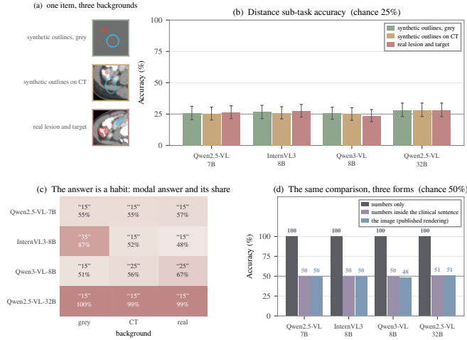
Fig. 5. Controls for distance estimation and numerical comparison. (a) One item under three backgrounds: synthetic outlines on grey, the same outlines over real anatomy with its annotations erased, and the real lesion and target. (b) Distance sub-task accuracy per model and background, volume-clustered 95% intervals. (c) The modal answer and its share: the habit does not change with what the outlines enclose. (d) The same comparison as two numbers, as those numbers inside the clinical sentence, and as the published image.
