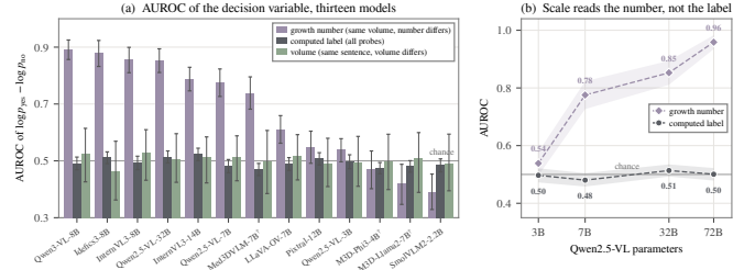
Fig. 6. Decision-score discrimination of growth values and computed labels. (a) AUROC of \log p_{\text{yes}} - \log p_{\text{no}} with volume-clustered 95% intervals: within matched pairs, where only the growth number differs; against the computed label; and across probes whose sentence is identical and only the volume differs. \dagger Native volumetric input. (b) The two AUROCs across Qwen2.5-VL 3B–72B.
