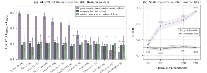
Fig. 7. The decision variable reads the question, not the volume. (a) AUROC of \log p_{\text{yes}} - \log p_{\text{no}} on the growth-matched subset with volume-clustered 95% intervals, three comparisons per model: within the 363 complete matched pairs, where volume and rendering are identical and only the growth number in the question differs; against the computed label over all 1,368 probes; and across the 182 probes whose question sentence is identical and only the volume differs. †Native volumetric input. (b) The growth-number and label AUROCs across Qwen2.5-VL 3B–72B on the published rendering.
