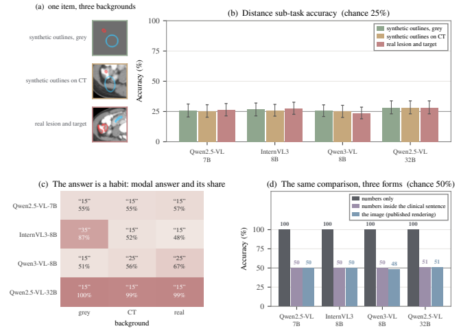
Fig. 5. Two ways the evidence contract breaks in the volume: a channel the models lack on any image, and a clinical sentence that disables the arithmetic they have. (a) One item under three backgrounds: synthetic outlines on uniform grey, the same outlines over real anatomy with its annotations erased, and the real lesion and target. (b) Distance sub-task accuracy per model and background, volume-clustered 95% intervals; synthetic gaps follow the real gap distribution and every gold is recomputed from the drawn masks. (c) The modal answer and its share: the habit does not change with what the outlines enclose. (d) The comparison the probe reduces to, posed as two numbers, as the same numbers inside the clinical sentence with no image, and as the published image.
