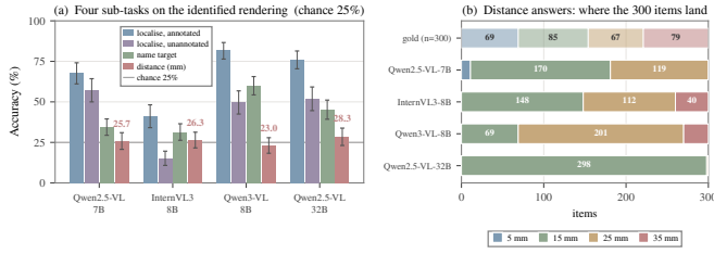
Fig. 4. Perception works, naming partly works, metric estimation is absent. (a) Sub-task accuracy on the identified rendering with volume-clustered 95% intervals: which organ holds the red-outlined lesion, the same with outlines and legend removed, which structure is outlined in cyan, and how many millimetres separate them. (b) Where the 300 distance answers land against the near-uniform gold: every model collapses onto one or two buckets, Qwen2.5-VL-32B onto “15” for 298 items.
