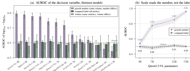
Fig. 6. The decision variable reads the question, not the volume. (a) AUROC of \log p_{\text{yes}} - \log p_{\text{no}} on the growth-matched subset with volume-clustered 95% intervals, three comparisons per model: within the 363 complete matched pairs, where volume and rendering are identical and only the growth number in the question differs; against the computed label over all 1,368 probes; and across the 182 probes whose question sentence is identical and only the volume differs. † Native volumetric input. (b) The growth-number and label AUROCs across Qwen2.5-VL 3B–72B on the published rendering.
