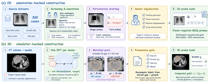
Fig. 2. Two constructions, one evaluation. (a) 2D, annotation-backed: 300 source cases from VQA-RAD, SLAKE, ROCO and chest radiograph collections; two radiologists screen and annotate each case (gold, A–E candidates, ROI, laterality, risk tier L1–L5); image and text perturbations are drafted as controlled variants of the same case; a senior radiologist finalises the gold keys, enforces the construction invariants and drops invalid probes. (b) 3D, simulator-backed: one Euclidean distance transform per lesion, computed with physical voxel spacing, gives the surface gap d to each target; a matched pair states one growth below the gap and one above it ( d = 10.2 mm, g^- = 8 , g^+ = 16 mm); a provenance gate recomputes every label y = 1[g \geq d] from the stored geometry. Both banks enter the shared evaluation of Section II-D.
