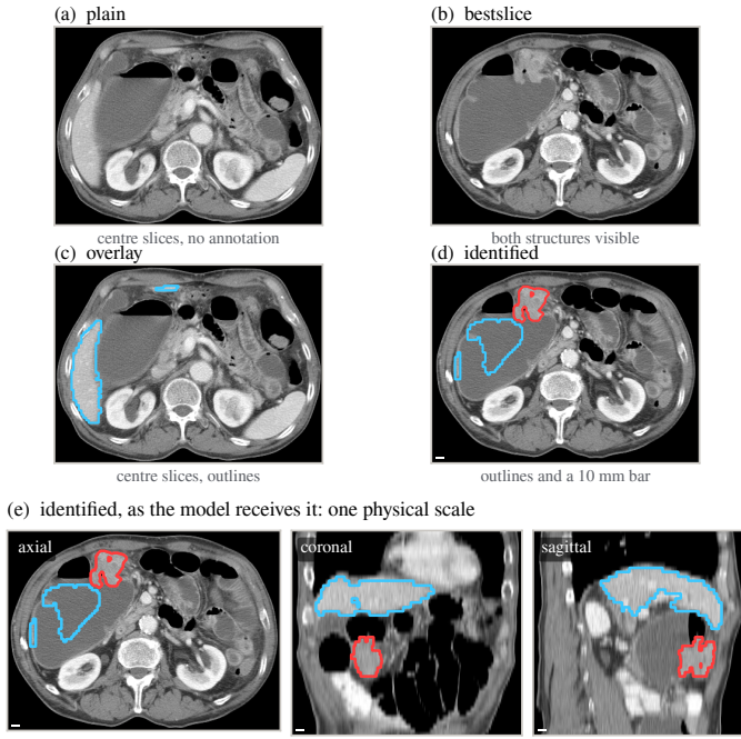
Fig. 3. What the volumetric models are shown. One growth-contact probe (colon, lesion 1, target liver; surface gap 3.97 mm). (a–d) The axial panel under the four identification conditions. The published plain input takes the three centre slices, on which the lesion the question names has no voxel, as for 42.0% of growth-matched probes; bestslice re-points the panels at slices showing both structures; overlay keeps the centre slices and adds the legend sentence, so the prompt describes an outline the image does not contain; identified combines joint-visibility slices, both outlines and a 10 mm bar, and is byte-identical to the reader-study rendering and to the input of the sub-task decomposition (Fig. 4). (e) The three identified panels as the model receives them, at one physical scale. Outlines are drawn as contours for display; the models receive 1-pixel outlines.
