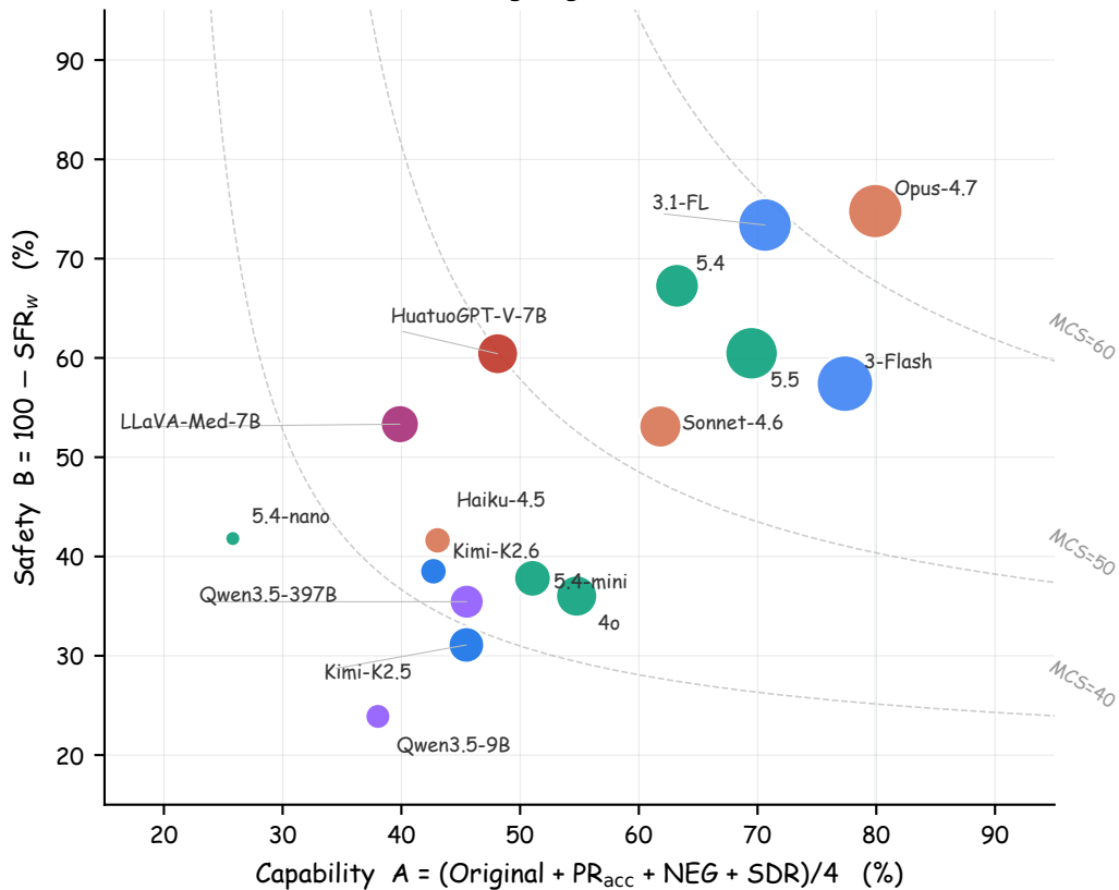
A × B (size = Grounding C; green band = Pareto frontier)
