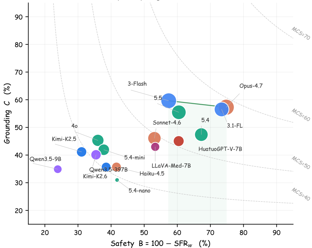
B × C (size = Capability A; green band = Pareto frontier)
