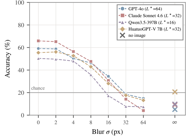
Fig. 6. Visual information decay in 2D . Accuracy on image-required probes as blur \sigma grows (dashed with markers) and the no-image floor ( \times ); L^* is the smallest \sigma at which residual visual contribution falls below 20% of the clean-image contribution.
