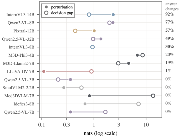
(b) Perturbation vs decision gap, per model
