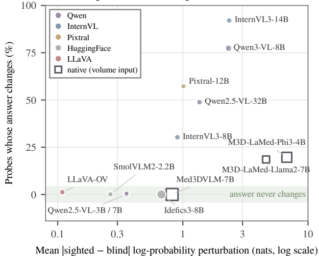
(a) Perturbation against answer change (marker area \propto decision gap)
