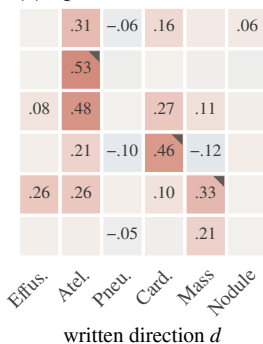
(b) Qwen2.5-VL-72B, NIH
