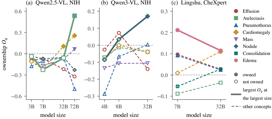
Figure 7: Size ladders. Ownership O_q per concept across sizes for Qwen2.5-VL on NIH, and Qwen3-VL on NIH, and Lingshu on CheXpert. The solid lines mark the concept with the largest ownership at the largest size is drawn as a thick solid line (Atelectasis, Nodule, Edema), the other concepts dashed; filled markers are owned cells. Each panel has its own vertical scales differ by panel.
