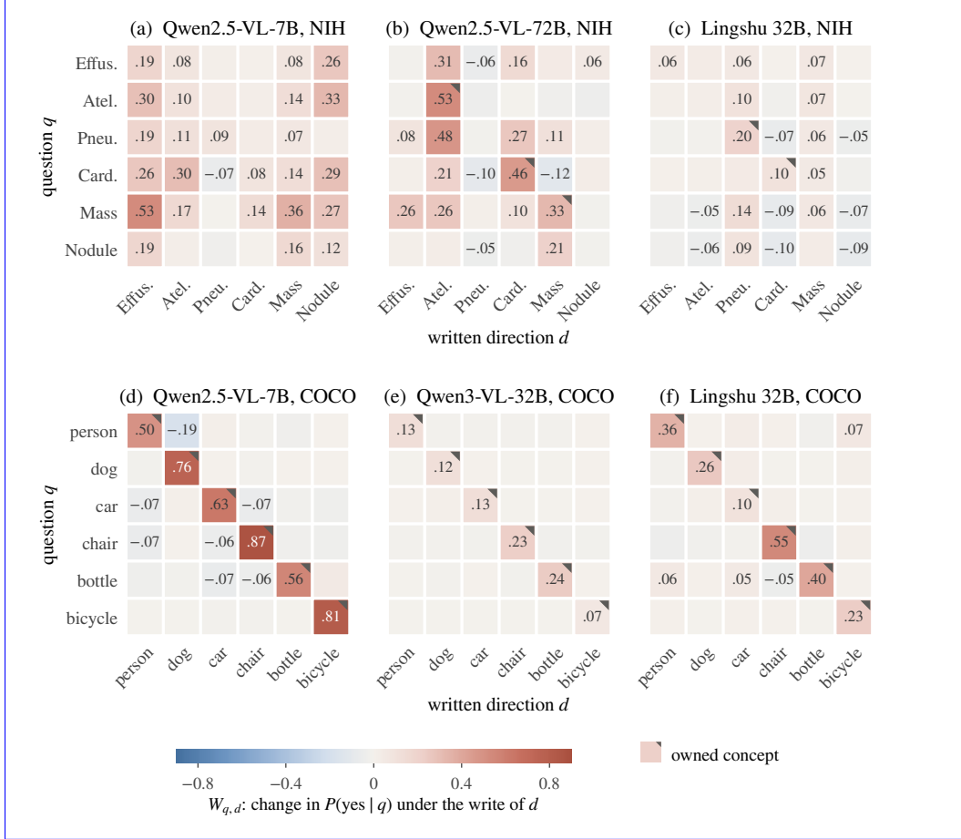
Figure 5: Write matrices. W_{q,d} , the mean change in P(\text{yes}) of question q (rows) under the write of direction d (columns), for three checkpoints on NIH (top) and three on COCO (bottom). A corner mark flags owned concepts.
