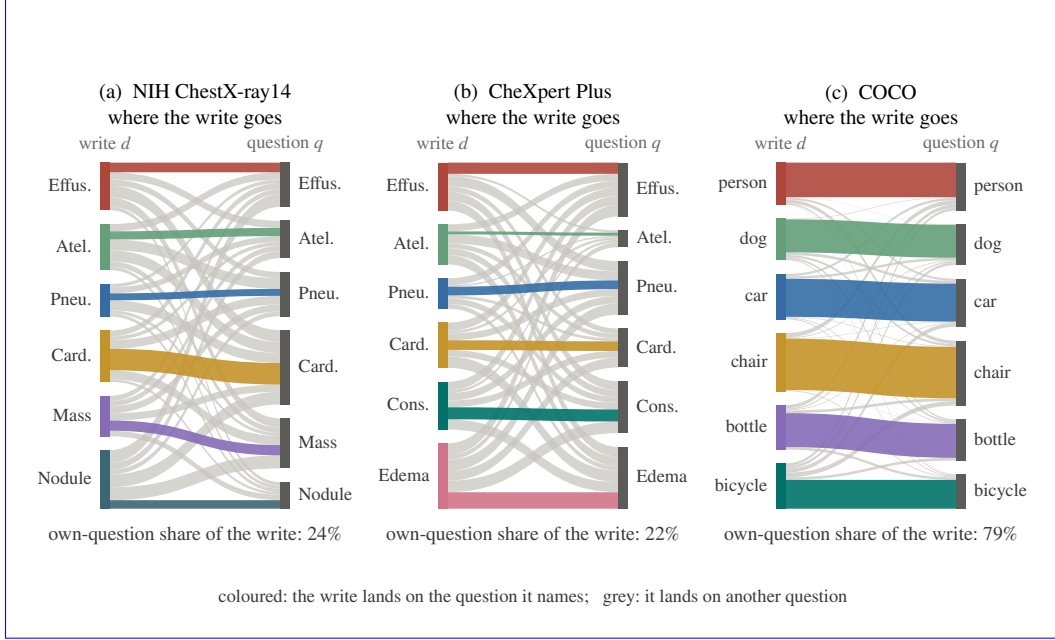
Figure 3: Where the write goes. Bands join each written direction d to the questions q it moves, with width proportional to F_{q,d} , the mean over checkpoints of \max(W_{q,d}, 0) . The percentage is the own-question share \sum_d F_{d,d} / \sum_{q,d} F_{q,d} .
