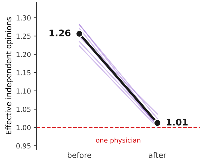
(a) Peer discussion
