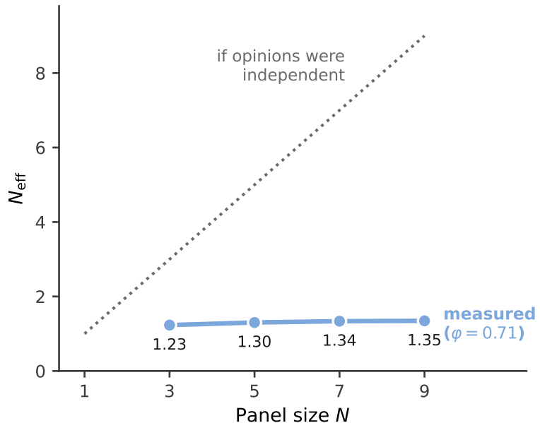
(b) Adding agents adds almost nothing
