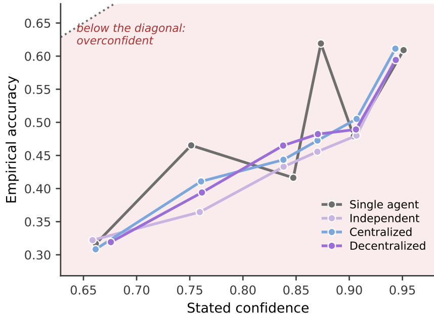
(a) Every architecture is overconfident
