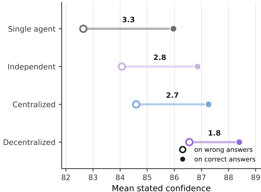
(b) Gap between wrong and right answers
