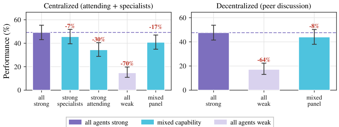
Figure 13: Agent heterogeneity. Performance of Centralized and Decentralized panels at n_a=3 on MedXpertQA under five capability placements. Strong is gpt-5-mini, weak is gpt-4.1-nano; strong specialists pairs a weak attending with strong specialists and strong attending reverses that pairing. Annotations give the change relative to the all-strong panel (dashed line). Decentralized coordination has no attending, so the two attending-capability conditions are structurally undefined there and are omitted.
