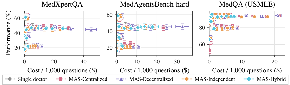
Figure 12: Cost-performance trade-offs. Mean performance against nominal cost per 1,000 questions, with SEM error bars on both axes. Each point is one configuration.
