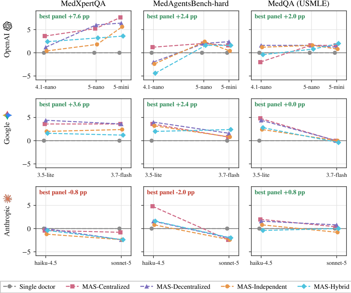
Figure 3: Agent scaling across model capability and system architecture. Gain over the single doctor, in percentage points, against the task-grounded capability index I (mean single-doctor accuracy across the three benchmarks); each architecture at its best-performing panel size. Rows are vendors, columns benchmarks, and all nine panels share one vertical scale, so magnitudes are comparable throughout. Plotting absolute accuracy instead would put the three benchmarks on ranges of 15–95% and collapse the architectures onto a single line: the effects being compared span -4.4 to +7.6 pp, while capability moves performance by tens of points. Every configuration sits inside a narrow band around the baseline, and the band narrows as the single doctor improves.
