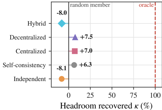
(b) How much of it any rule recovers
