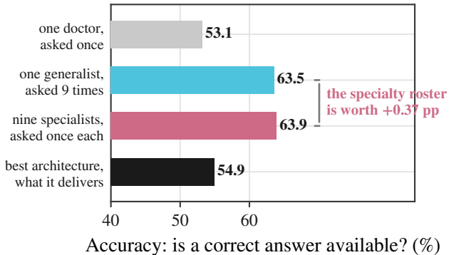
(a) Nine specialists \approx one generalist asked nine times
