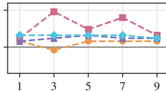
MedAgentsBench-hard
