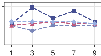
MedAgentsBench-hard
