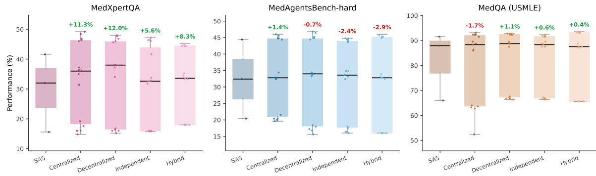
Figure 4: Single-agent versus multi-agent performance distributions. Box plots over all configurations of each architecture, with individual configurations overlaid. Annotations give the change in mean relative to the single-agent baseline.
