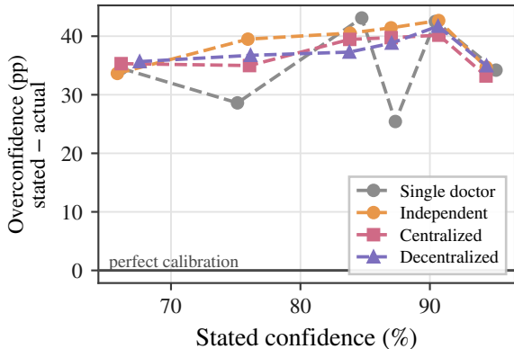
(a) Every architecture overstates itself
