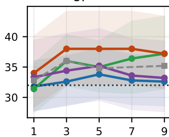
T2 gpt-5-nano
