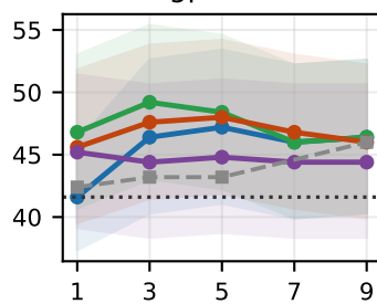
T3 gpt-5-mini
