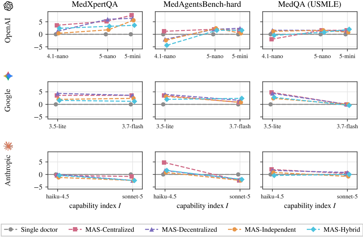
Figure 2: Agent scaling across model capability and system architecture. Gain over the single doctor, in percentage points, against the task-grounded capability index I (mean single-doctor accuracy across the three benchmarks); each architecture at its best-performing panel size. Rows are vendors, columns benchmarks, and all nine panels share one vertical scale, so magnitudes are comparable throughout. Plotting absolute accuracy instead would put the three benchmarks on ranges of 15–95% and collapse the architectures onto a single line: the effects being compared span -4.4 to +7.6 pp, while capability moves performance by tens of points. Every configuration sits inside a narrow band around the baseline, and the band narrows as the single doctor improves.
