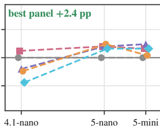
MedAgentsBench-hard
