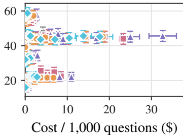
MedAgentsBench-hard
