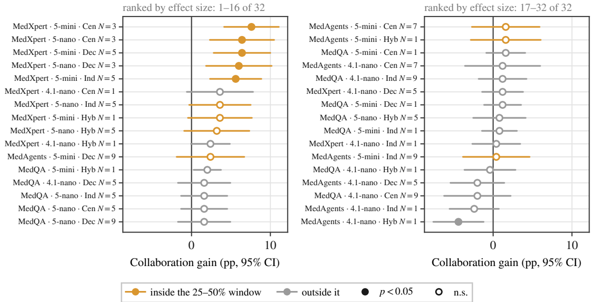
Figure 13: Effect size for every configuration, ranked. Collaboration gain with 95% confidence intervals; each row is one architecture at its best panel size within a difficulty stratum, and rows run left to right in descending order of effect. Amber rows have a single-doctor baseline inside the 25–50% window, grey rows outside it. Filled markers are significant at p < 0.05 , hollow are not. The ranking is what carries the claim: amber occupies the positive tail and grey the negative one, and every significant row on the positive side is amber while the only significant row on the negative side is grey.
