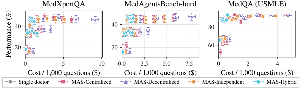
Figure 11: Cost-performance trade-offs. Mean performance against nominal cost per 1,000 questions, with SEM error bars on both axes. Each point is one configuration.
