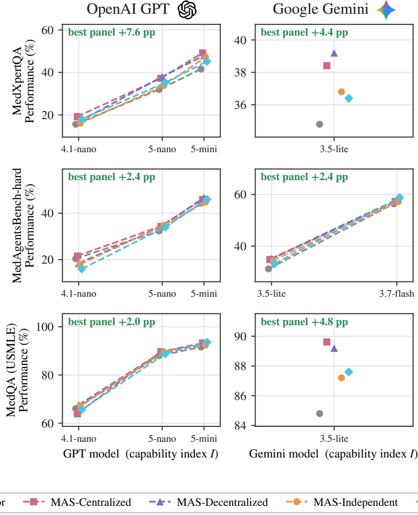
Figure 3: Agent scaling across model capability and system architecture. Top: performance against the task-grounded capability index I (mean single-doctor accuracy across the three benchmarks), each architecture at its best-performing panel size, grey the single doctor. Ticks mark the three GPT tiers at their measured I of 34.0, 50.8 and 59.2, and the corner figure is the best architecture’s gain at the strongest model. The three benchmarks occupy different accuracy ranges, so the bottom row replots the same configurations as gain over the single doctor on one shared scale, where architecture effects are directly comparable across benchmarks. They span -4 to +8 pp while capability moves performance by tens of points.
