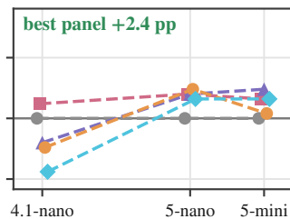
MedAgentsBench-hard
