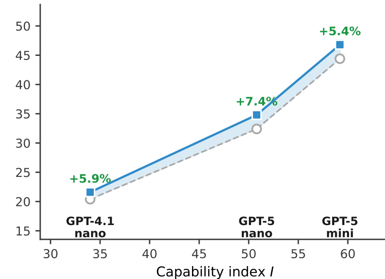
MedAgentsBench-hard
