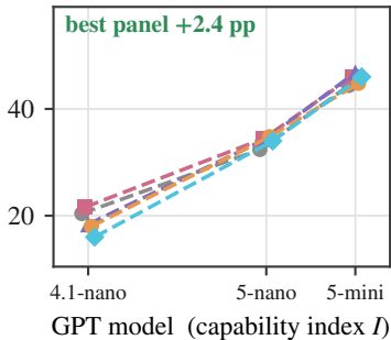
MedAgentsBench-hard
