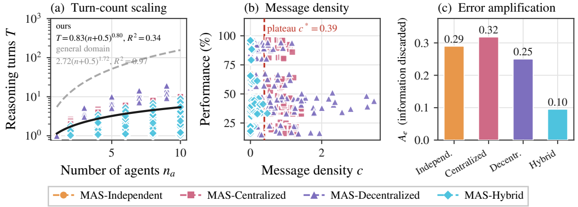
Figure 9: A panel discards what it holds. (c) Error amplification A_e : the share of correct first opinions a panel emits a wrong answer over, normalised by the single-agent error rate. (a) and (b) place the setting against the published general-domain law: medical panels converse an order of magnitude less than it predicts, and performance is uncorrelated with how much the panel says (§G).
