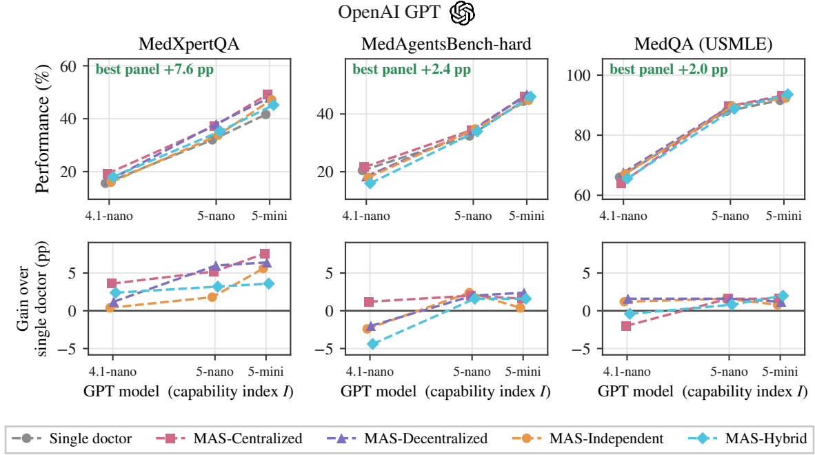
Figure 3: Agent scaling across model capability and system architecture. Top: performance against the task-grounded capability index I (mean single-doctor accuracy across the three benchmarks), each architecture at its best-performing panel size, grey the single doctor. Ticks mark the three GPT tiers at their measured I of 34.0, 50.8 and 59.2, and the corner figure is the best architecture’s gain at the strongest model. The three benchmarks occupy different accuracy ranges, so the bottom row replots the same configurations as gain over the single doctor on one shared scale, where architecture effects are directly comparable across benchmarks. They span -4 to +8 pp while capability moves performance by tens of points.
