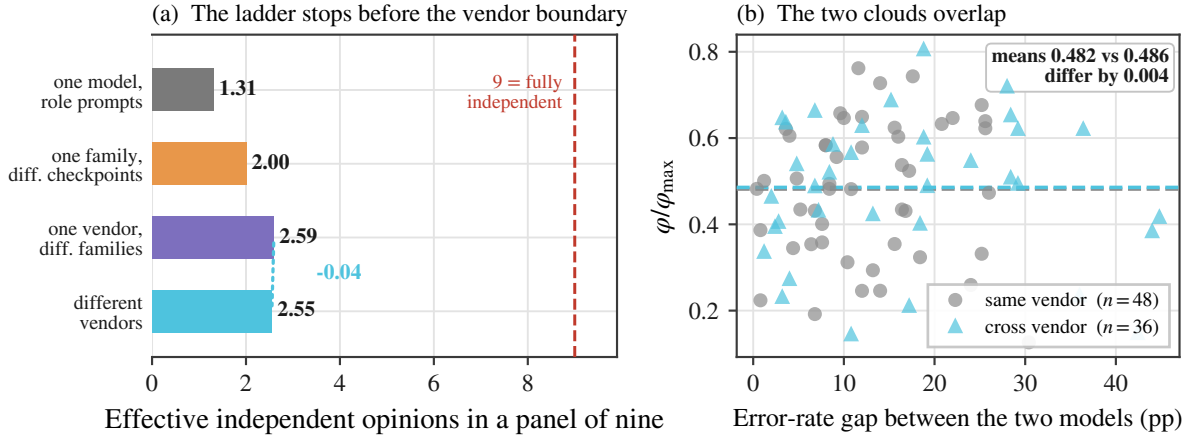
Figure 6: Independence does not arrive at the vendor boundary. (a) Effective independent opinions in a nine-member panel under four sources of diversity. Relaxing the prompt, then the checkpoint, then the training family lifts the panel from 1.31 to 2.59; relaxing the vendor moves it -0.04 . (b) The evidence behind that mean: all 84 model pairs, normalised correlation against the gap in the two members’ error rates. The same-vendor and cross-vendor clouds occupy the same region and their means differ by 0.004. The rightward drift of both is Eq. 3 at work, which is why the normalised quantity is the one plotted.
