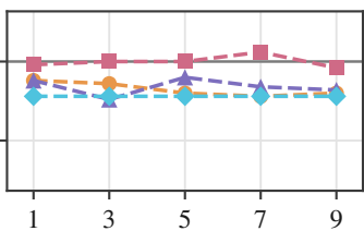
MedAgentsBench-hard
