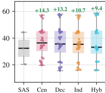
MedAgentsBench-hard
