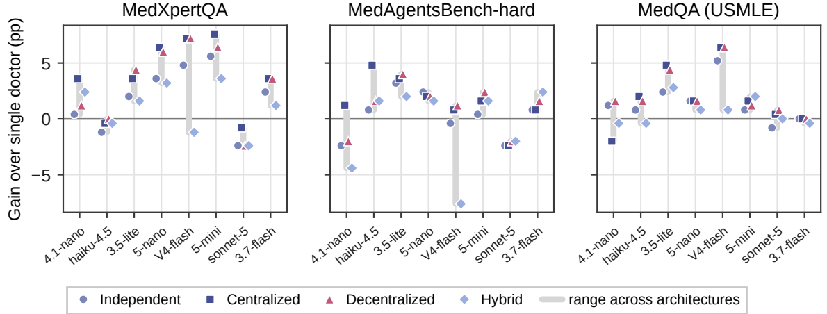
Figure 6: Every architecture lands close to the single doctor. Each panel shows a benchmark. The eight models are ordered by I , their mean single-doctor accuracy across benchmarks. Markers show each architecture’s gain (pp) at its best panel size; grey bars span the four architectures. Figure 7 gives the vendor breakdown.
