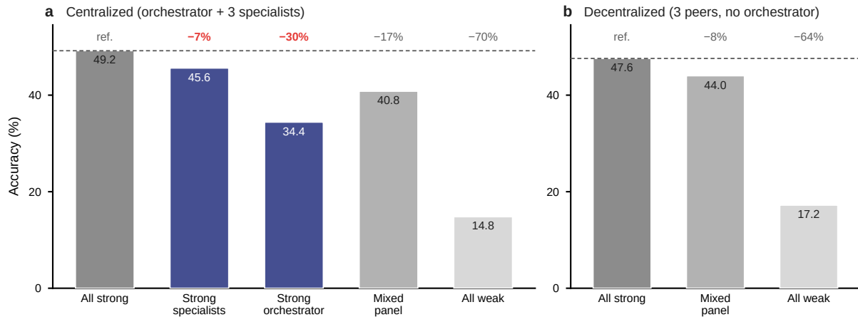
Figure 12: Agent heterogeneity. Bars show one run’s accuracy on 250 MedXpertQA questions at N = 3 . Strong is gpt-5-mini; weak is gpt-4.1-nano; mixed panels also use gpt-5-nano. Strong specialists pairs a weak orchestrator with strong specialists; strong orchestrator reverses this. Decentralized has no orchestrator. Dashed lines mark all-strong panels; top-row percentages give relative changes.
