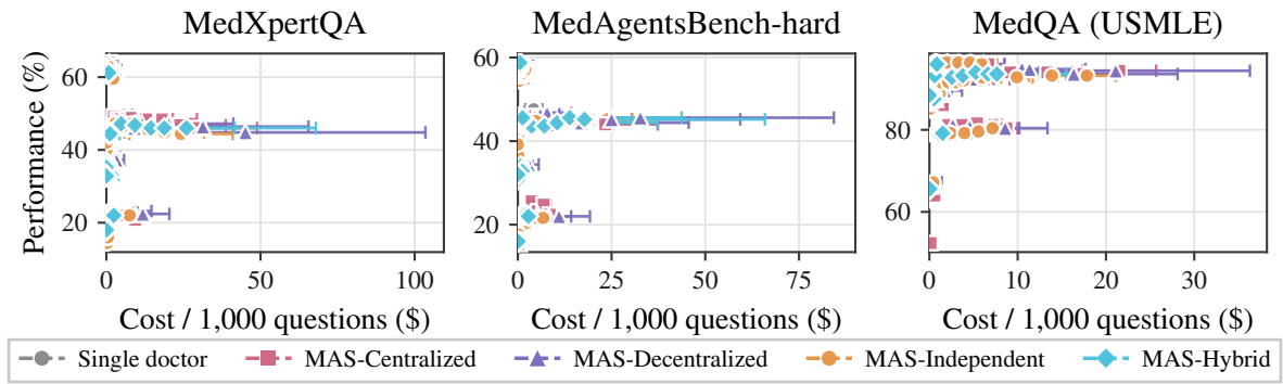
Figure 13: Cost–performance trade-offs. Mean performance is plotted against nominal cost per 1,000 questions, with standard-deviation bars on the cost axis. Each point is one configuration.
