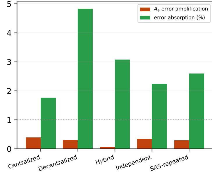
(c) error dynamics by architecture
