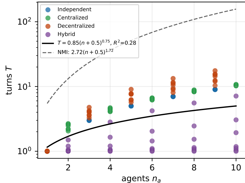
(a) turn-count power law
