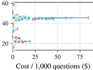
MedAgentsBench-hard
