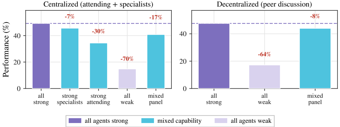
Figure 14: Agent heterogeneity. MedXpertQA performance is shown at n_a=3 . The strong model is gpt-5-mini and the weak model is gpt-4.1-nano. Strong specialists pairs a weak attending with strong specialists; strong attending reverses this pairing. Annotations give percentage changes relative to the all-strong dashed line. Decentralized coordination has no attending.
