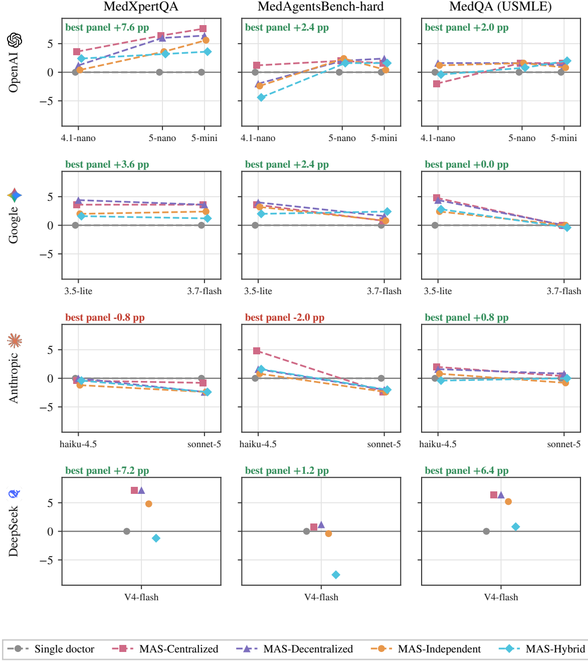
Figure 9: The capability grid in full. Figure 3’s gains share one scale (pp) across vendor rows and benchmark columns; models are positioned by I . Grey shows the single doctor at zero. Coloured annotations give each vendor’s strongest model’s best gain.
