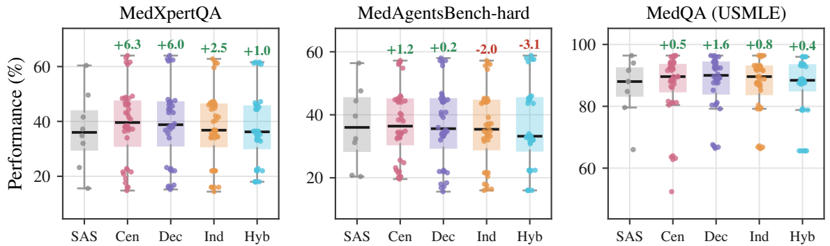
Figure 12: Single doctor versus panel: performance distributions. Box plots show configuration accuracies, with individual configurations overlaid. The bars are labelled SAS (single doctor), Cen (Centralized), Dec (Decentralized), Ind (Independent) and Hyb (Hybrid). Annotations give changes in mean accuracy as percentages of the single-doctor baseline.
