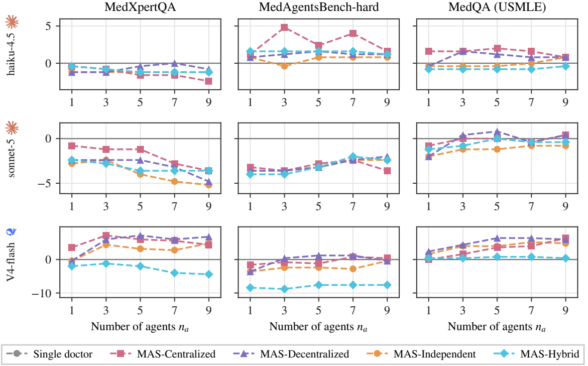
Figure 11: Number-of-agents scaling, Anthropic and DeepSeek. As Figure 10, for the remaining three models.
