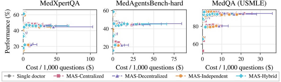
Figure 13: Cost-performance trade-offs. Mean performance is plotted against nominal cost per 1,000 questions, with SEM error bars on both axes. Each point is one configuration.
