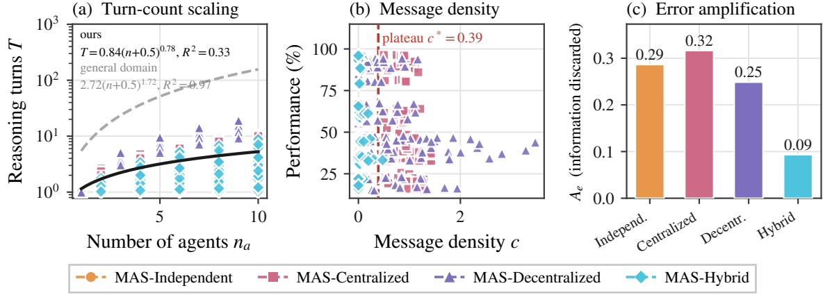
Figure 8: A panel discards what it holds. (c) Error amplification A_e measures the share of available correct first opinions lost to a wrong output, normalised by the single-agent error rate. Panels (a) and (b) compare turn counts and message density with the published general-domain law.
