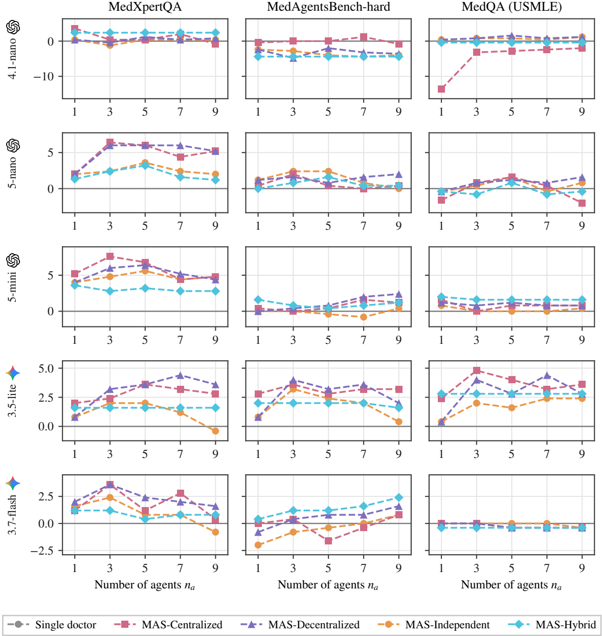
Figure 10: Number-of-agents scaling, OpenAI and Google. Gain over the single doctor (pp) is plotted against n_a for each architecture. Rows are models, columns are benchmarks, and each row shares a vertical scale. Figure 11 covers Anthropic and DeepSeek.
