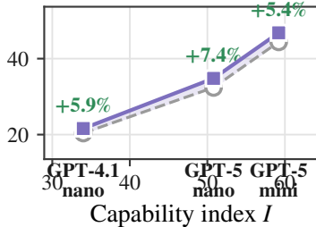
MedAgentsBench-hard
