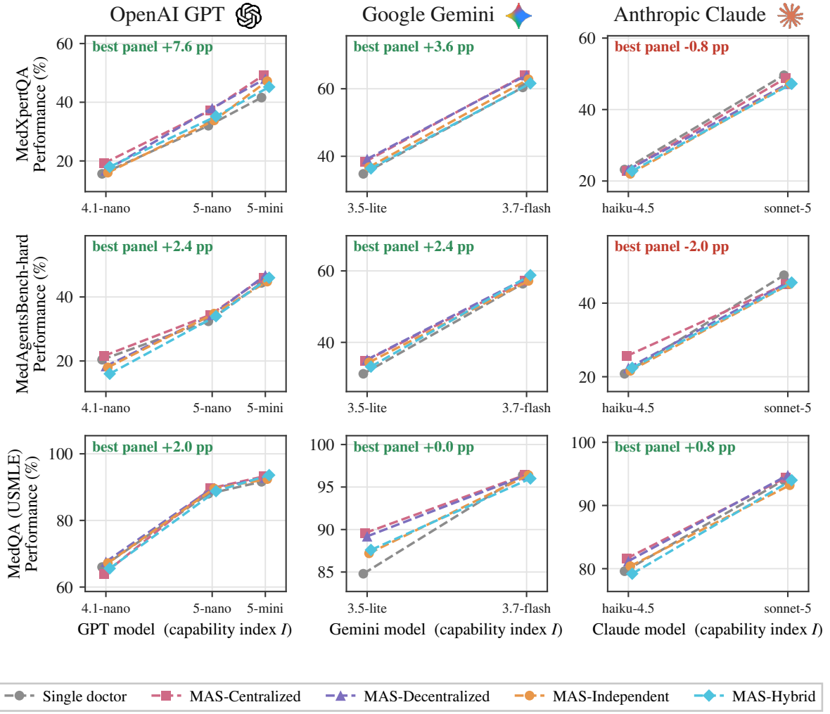
Figure 2: Agent scaling across model capability and system architecture. Top: performance against the task-grounded capability index I (mean single-doctor accuracy across the three benchmarks), each architecture at its best-performing panel size in grey the single doctor. Ticks mark the three GPT tiers at their measured I of 34.0, 50.8 and 59.2, and the corner figure is the best architecture’s gain at the strongest model. The three benchmarks occupy different accuracy ranges, so the bottom row replots the same configurations as gain over the single doctor on one shared scale, where architecture effects are directly comparable across benchmarks. They span -4 to +8 pp while capability moves performance by tens of points.
