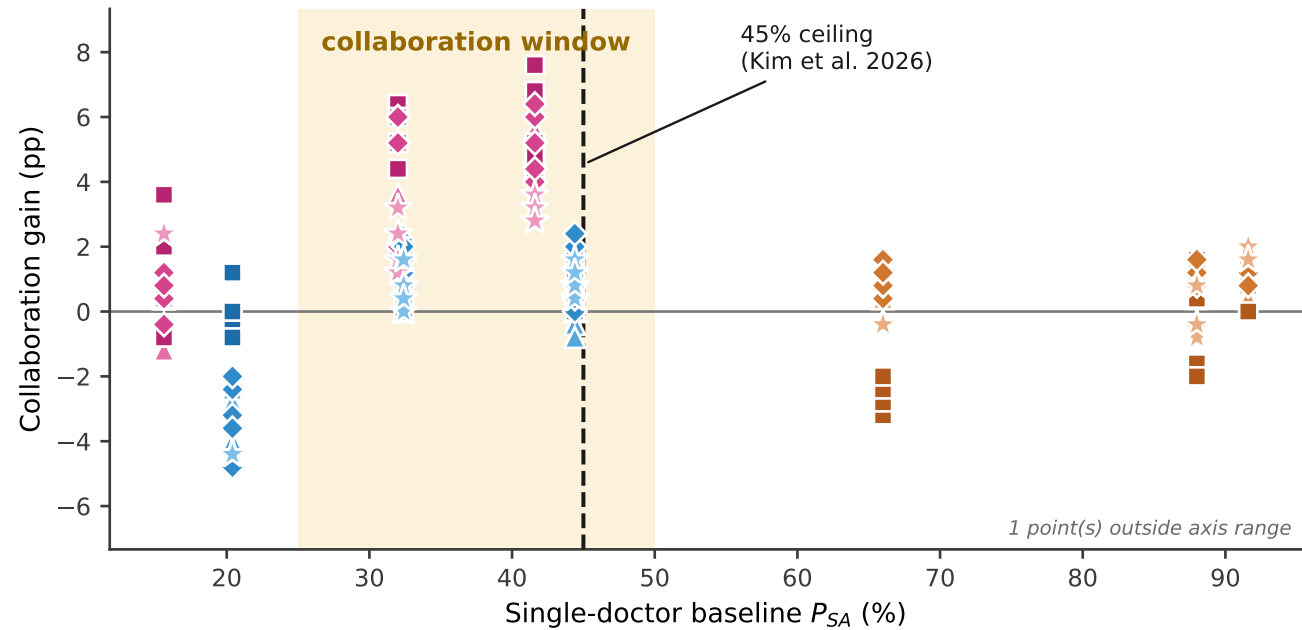
(a) Gain against single-agent baseline
