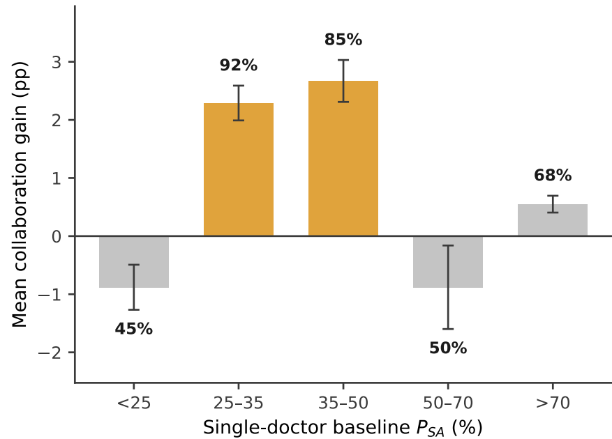
(b) Binned, with % of configurations that gain
