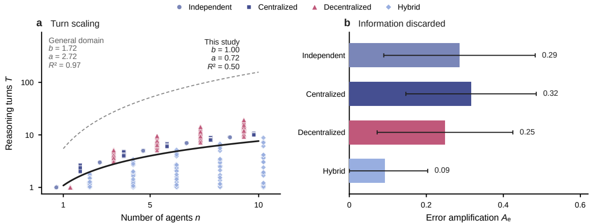
Figure 7: A panel discards what it holds. (a) Multi-agent configurations plot turns T against n (orchestrator included). The solid line fits T = a(n + 0.5)^b ; dashes give the general-domain law. (b) Bars show mean \pm SD across configurations by architecture; lower whiskers truncate at zero ( A_e \geq 0 ). A_e measures episodes losing correct first-round answers to wrong outputs, normalised by first-round agents’ error rate.
