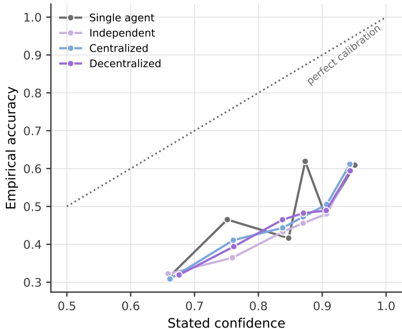
(a) Reliability
