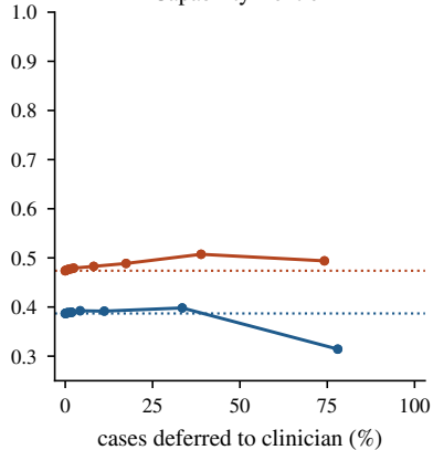
Capability frontier
