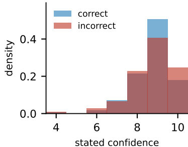
Capability frontier
