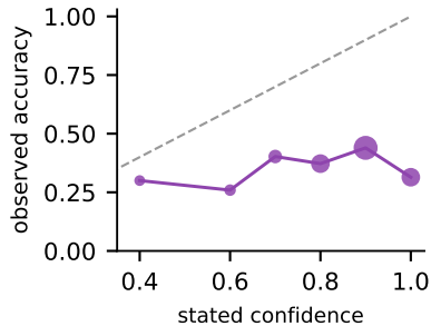
Capability frontier ECE=0.486
