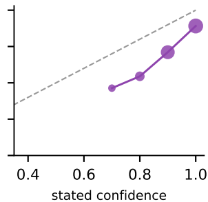
Standard difficulty ECE=0.162
