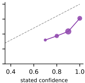
High acuity ECE=0.319
